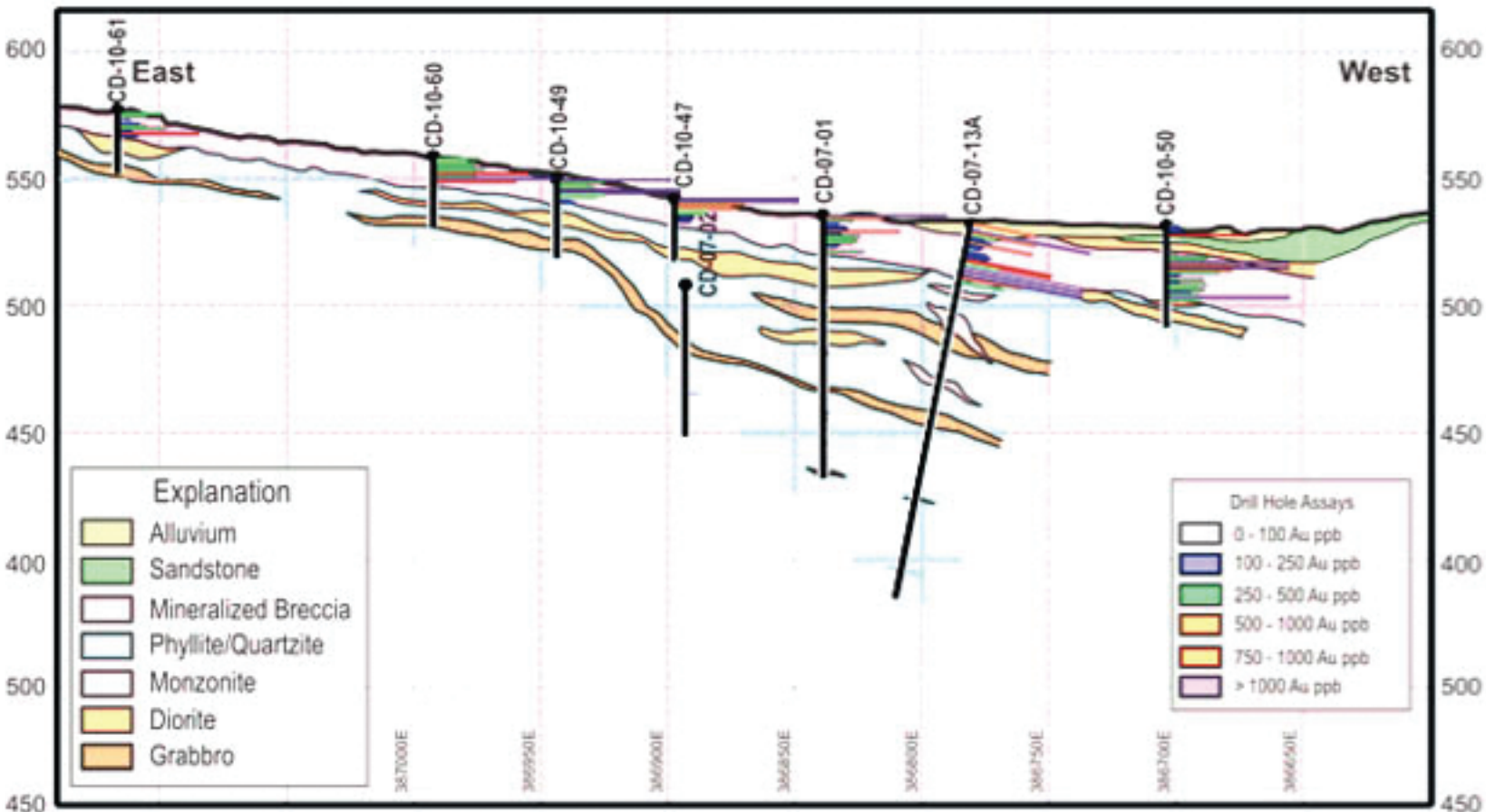
Canasta Cross Section 3418780N Looking South Sonora, Mexico
