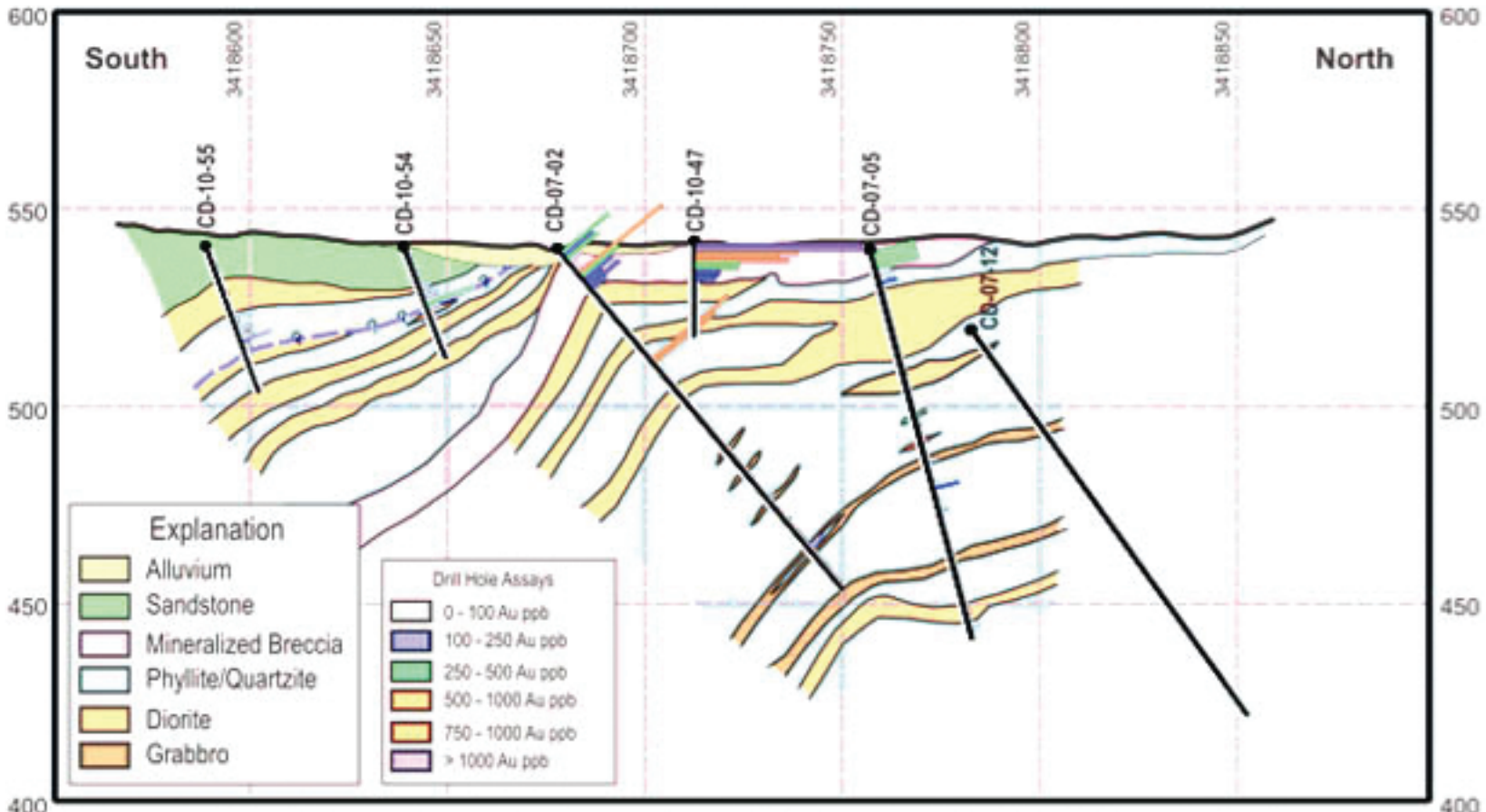
Canasta Cross Section 386900E Looking West Sonora, Mexico
